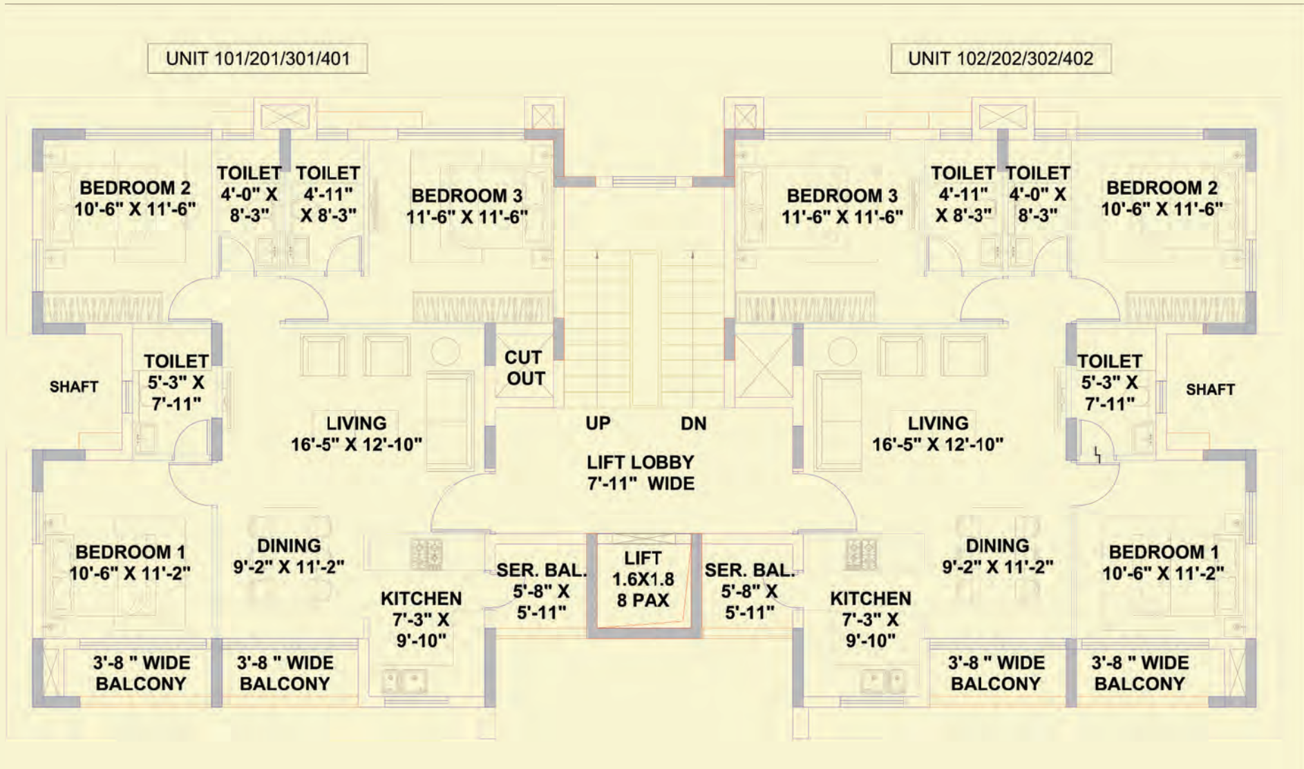
BUILDING - 3 (BLOCK 5) TYPICAL FLOOR PLAN
