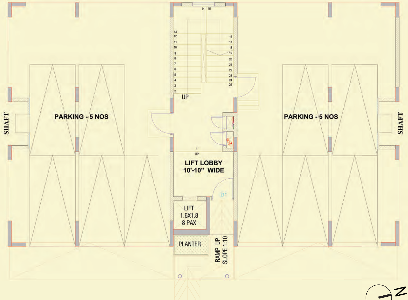
BUILDING - 1 (BLOCK 1- 4) GROUND FLOOR PLAN
