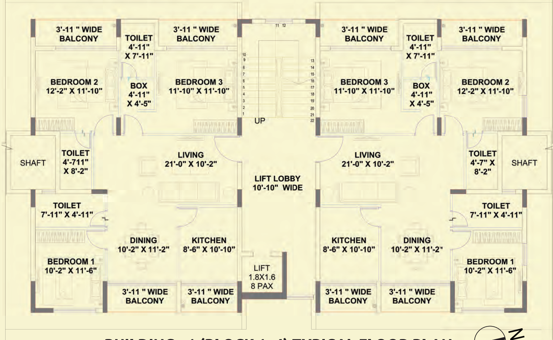
BUILDING - 1 (BLOCK 1- 4) TYPICAL FLOOR PLAN
